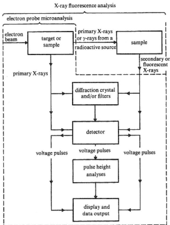
Figure 8.37 Schematic representation of X-ray emission spectrometry.
