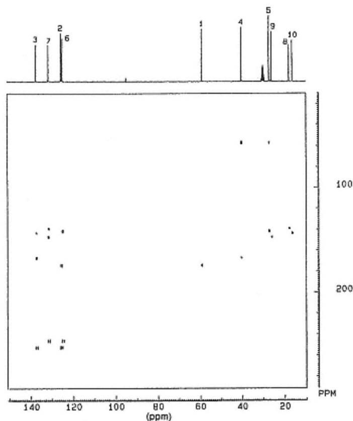
Figure 9.47 The INADEQUATE spectrum of geraniol in \text{CD}_3\text{COCD}_3 at 75.6 MHz for ^{13}\text{C} .
