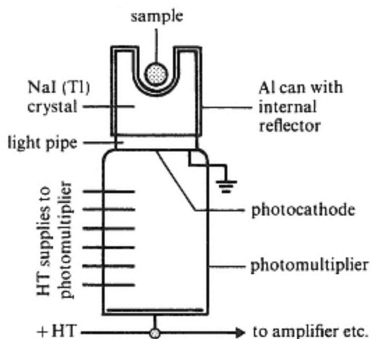
Figure 10.10 A typical scintillation detector. (Well crystal NaI).
