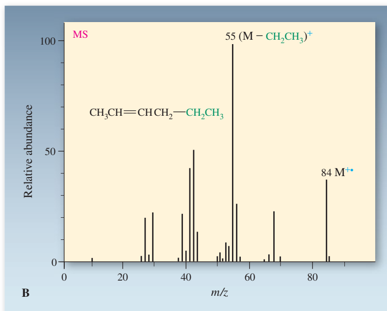
Figure 11-29 Mass spectra of (A) 1-butene, showing a peak at m/z = 41 from cleavage to give the resonance-stabilized 2-propenyl (allyl) cation; (B) 2-hexene, showing similar cleavage between C4 and C5 to give the 2-butenyl cation, with m/z = 55 .
