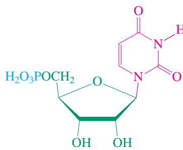
Uridylic acid
