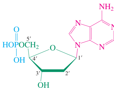
2'-Deoxyadenylic acid
