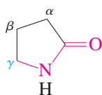
\gamma -Butyrolactam (Systematic name: aza-2-cyclopentanone)
