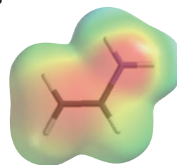
Ethenamine
