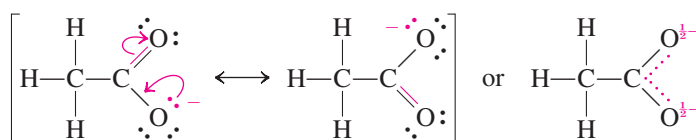
Acetate ion
