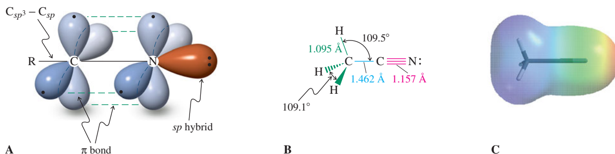
Figure 20-3 (A) Orbital picture of the nitrile group, showing the sp hybridization of both atoms in the \text{C}\equiv\text{N} function. (B) Molecular structure of ethanenitrile (acetonitrile), which is similar to that of the corresponding alkyne. (C) Electrostatic potential map of ethanenitrile, depicting the positively polarized cyano carbon (blue) and the relatively negatively polarized nitrogen (green) with its lone electron pair (red).
