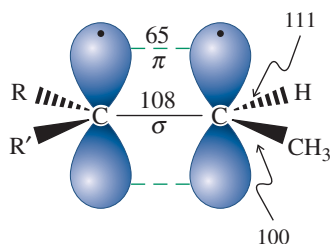
Figure 11-7 Approximate bond strengths in an alkene (in kcal mol -1 ). Note the relative weakness of the \pi bond.
