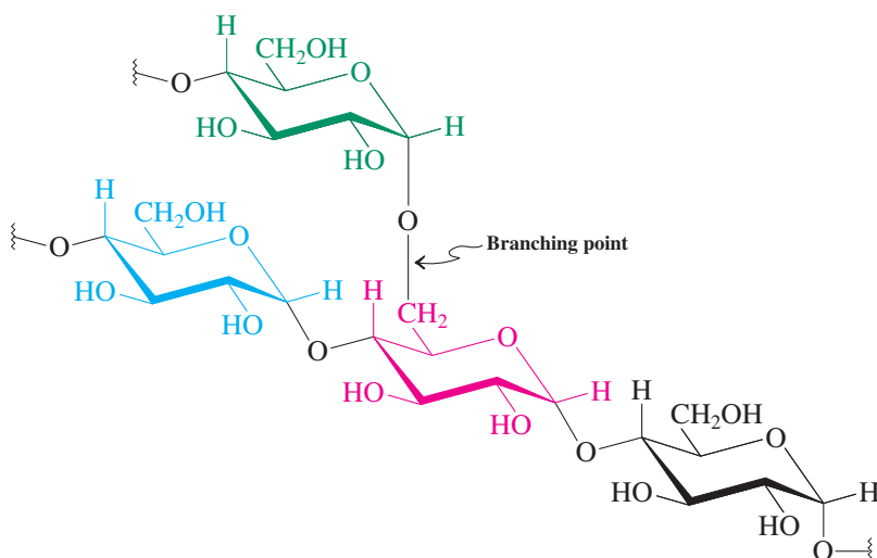
Amylopectin
