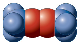
Dimethylacetylene
