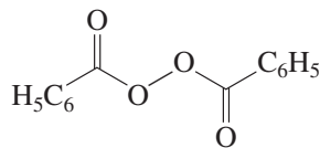
Dibenzoyl peroxide
