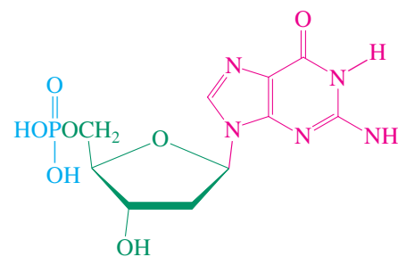
2'-Deoxyguanylic acid
