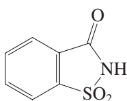
Compound C
