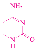
Cytosine (C)
