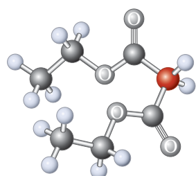
Diethyl propanedioate (Diethyl malonate)
