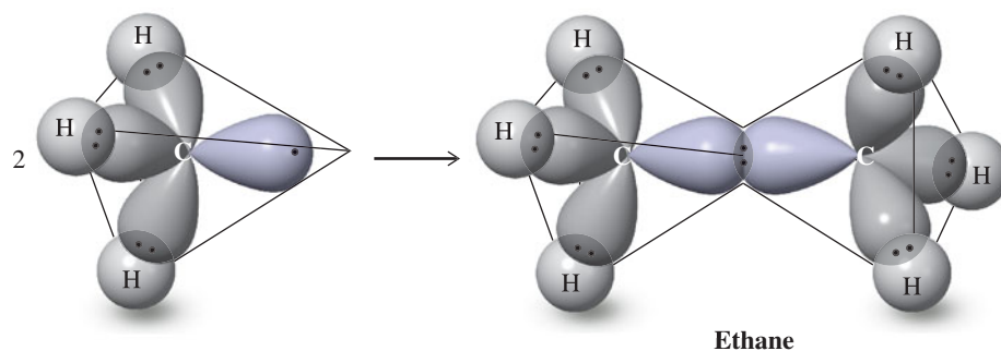
Figure 1-19 Overlap of two sp^3 orbitals to form the carbon–carbon bond in ethane.
