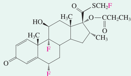
Fluticasone propionate
