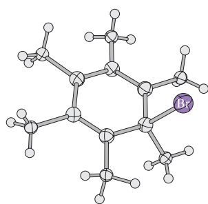
Figure 15-21 X-ray structure of the carbocation arising from attack of bromine on hexamethylbenzene. This cation can be isolated because it is unusually stabilized by the methyl substituents and because it lacks a proton on the sp^3 -hybridized carbon, thus disabling bromoarene formation.
