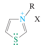
Thiazolium salt
