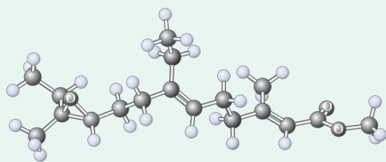
Juvenile hormone
