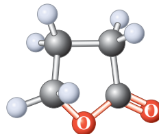
\gamma -Butyrolactone (Systematic: oxa-2-cyclopentanone)
