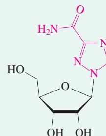
1-β-D-Ribofuranosyl-1,2,4-triazole-3-carboxamide (Ribavirin)
