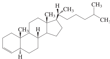
3-Cholestene
