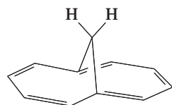
1,6-Methano[10]annulene
