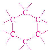
A carbocycle
