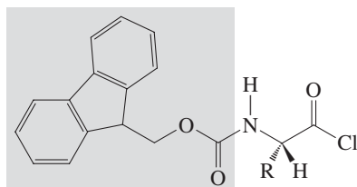
Fluorenylmethyloxycarbonyl (Fmoc)-amino acid chloride
