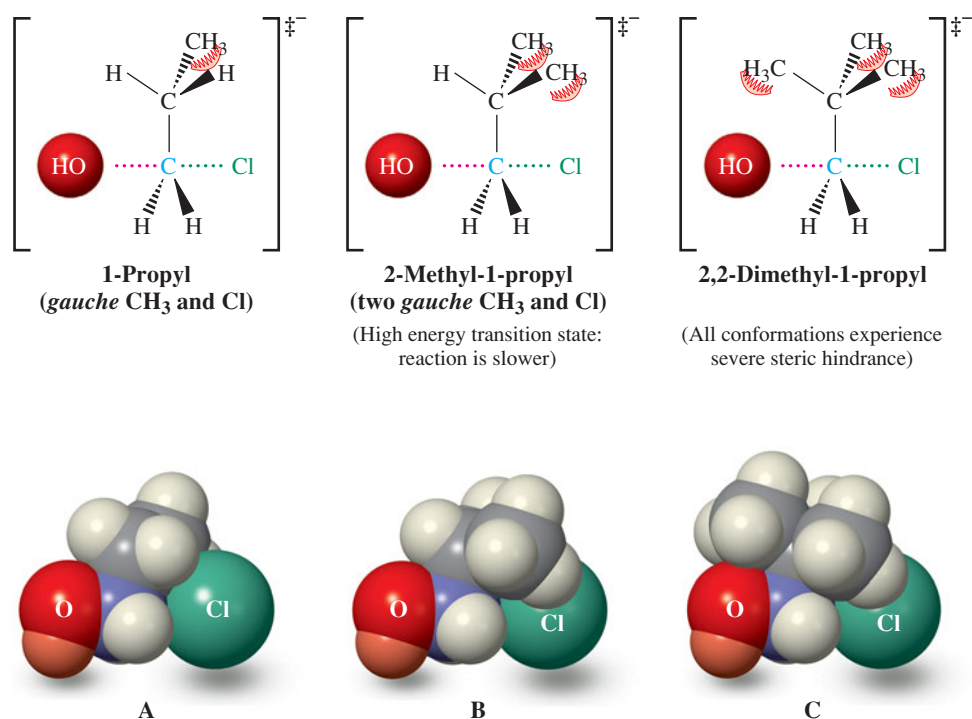
Figure 6-10 Hashed-wedged line and space-filling renditions of the transition states for S N 2 reactions of hydroxide ion with (A) 1-chloropropane, (B) 1-chloro-2-methylpropane, and (C) 1-chloro-2,2-dimethylpropane. Increasing steric hindrance from a second gauche interaction reduces the rate of reaction in (B). S N 2 reactivity in (C) is eliminated almost entirely because a methyl group prevents backside attack by the nucleophile in all accessible conformations of the substrate. (See also Figures 6-8 and 6-9.)
