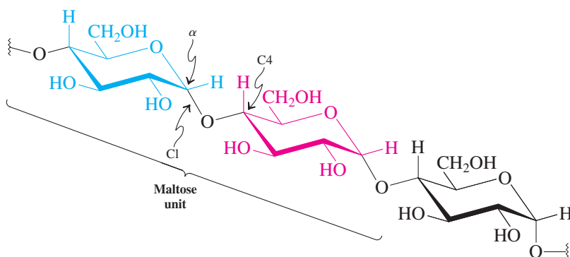
Amylose
