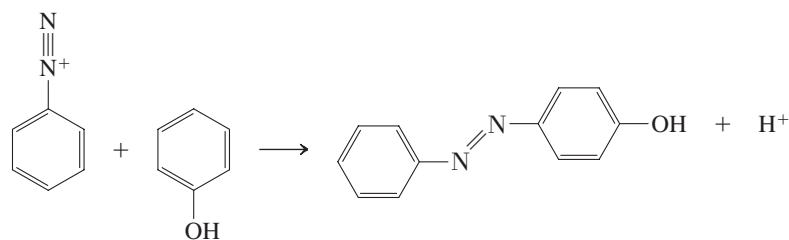
Azo compound
