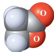
\beta -Propiolactone
