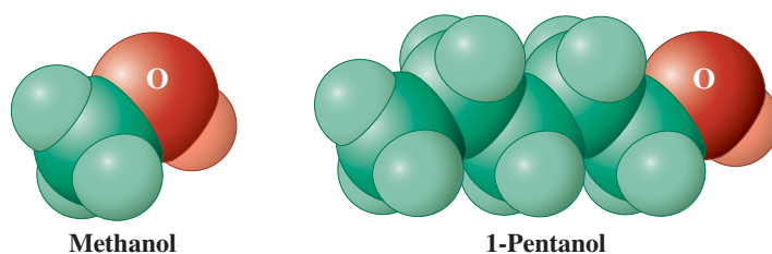
Figure 8-3 The hydrophobic and hydrophilic parts of methanol and 1-pentanol (space-filling models). The polar functional group dominates the physical properties of methanol: The molecule is completely soluble in water but only partially so in hexane. Conversely, the increased size of the hydrophobic part in 1-pentanol leads to infinite solubility in hexane but reduced solubility in water (Table 8-1).
