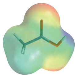
Acetic acid
