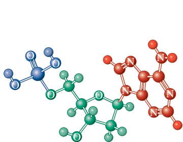
2'-Deoxyadenylic acid
