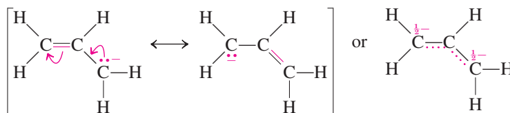
2-Propenyl (allyl) anion
