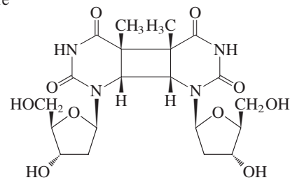
Thymidine dimer
