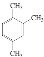
1,2,4-Trimethylbenzene
