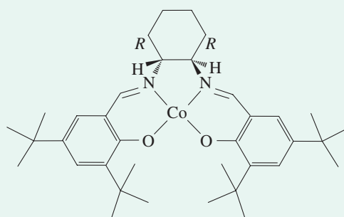
Cobalt catalyst
