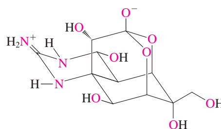
Tetrodotoxin (The nerve toxin in puffer fish or fugu)
