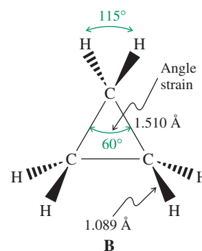
Figure 4-1 Cyclopropane: (A) molecular model; (B) bond lengths and angles.
