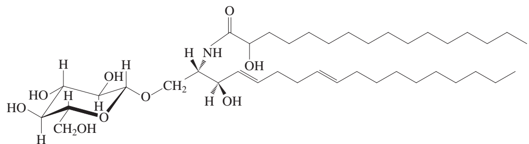
Glucosyl cerebroside
