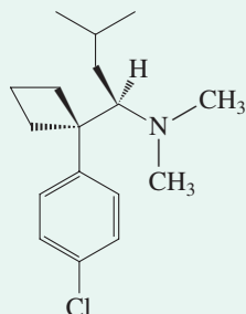
Sibutramine (Meridia)
