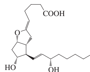
Prostacyclin I_2
