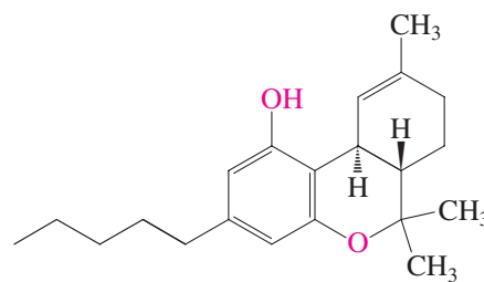
Tetrahydrocannabinol
