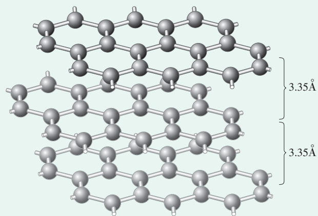
Graphite
