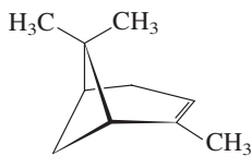
\alpha -Pinene
