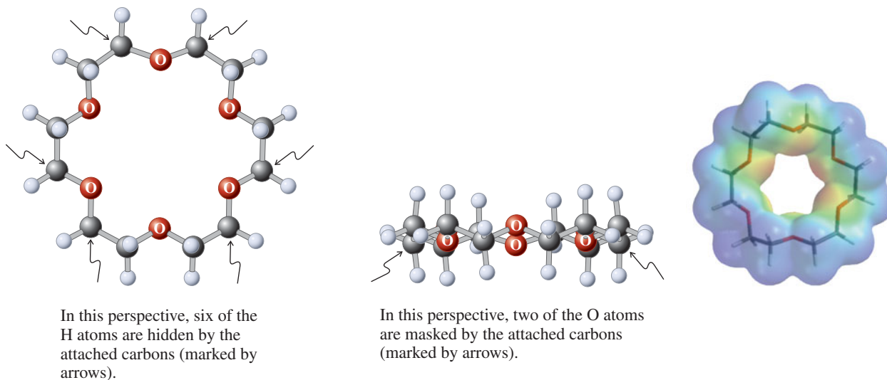
Figure 9-3 The crownlike structural arrangement of 18-crown-6.
