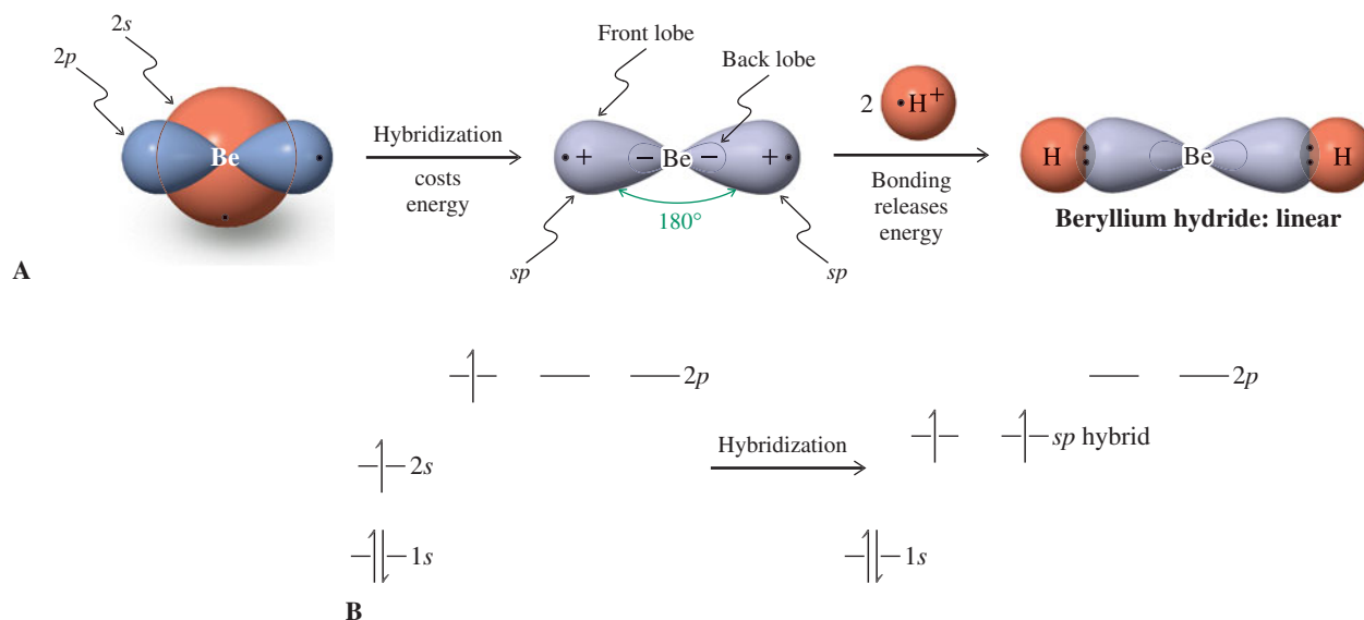
Figure 1-16 Hybridization in beryllium to create two sp hybrids. (A) The resulting bonding gives \text{BeH}_2 a linear structure. Again, both remaining p orbitals and the 1s orbital have been omitted for clarity. The sign of the wave function for the large sp lobes is opposite that for the small lobes. (B) The energy changes occurring on hybridization. The 2s orbital and one 2p orbital combine into two sp hybrids of intermediate energy. The 1s and remaining 2p energies remain the same.
