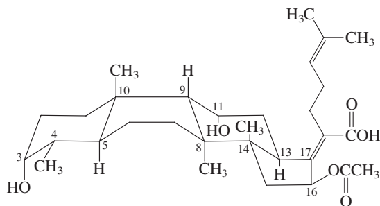
Fusidic acid
