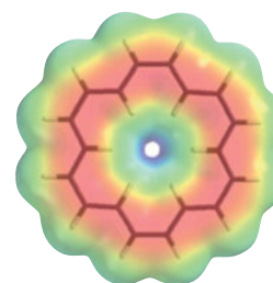
[18]Annulene: aromatic
