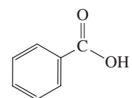
Benzoic acid
