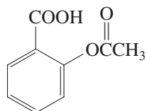
2-Acetoxybenzoic acid (Aspirin)
