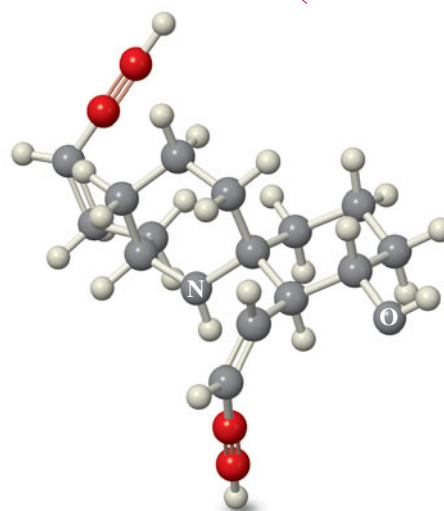
Histrionicotoxin
