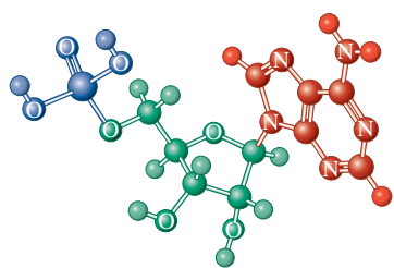
Adenylic acid
