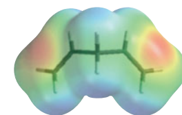
1,4-Pentadiene (Nonconjugated)
