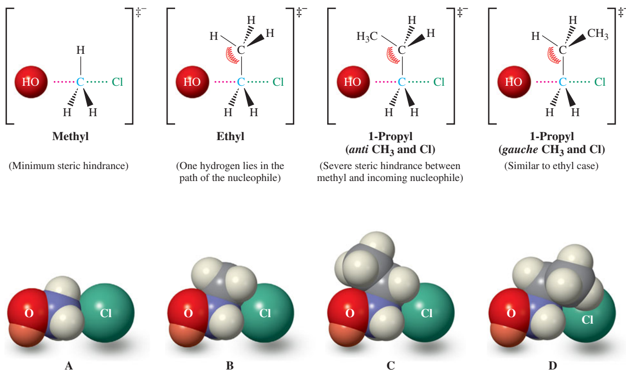
Figure 6-9 Hashed-wedged line and space-filling drawings of the transition states for S_N2 reactions of hydroxide ion with (A) chloromethane; (B) chloroethane; and (C and D) two conformers of 1-chloropropane: (C) anti and (D) gauche . Steric interference is illustrated strikingly in the space-filling drawings. Partial charges have been omitted for clarity. (See Figure 6-3.)
