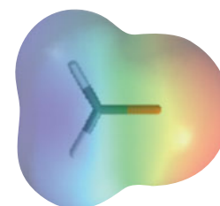
Formaldehyde
