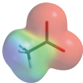
Acetate ion
