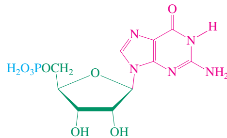
Guanylic acid
