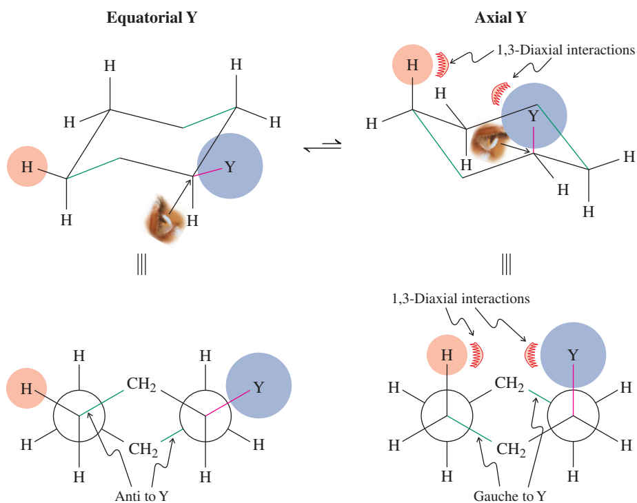
Figure 4-12 A Newman projection of a substituted cyclohexane. The conformation with an axial Y substituent is less stable because of 1,3-diaxial interactions, only one of which is shown (see the “eye” for the choice of the Newman projection). Axial Y is gauche to the ring bonds shown in green; equatorial Y is anti .
