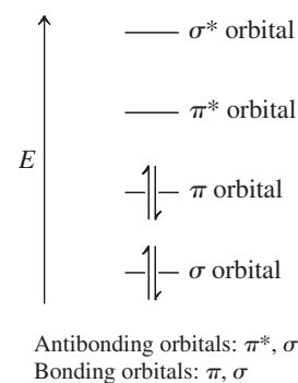
Figure 11-5 Energy ordering of the molecular orbitals making up the double bond. The four electrons occupy only bonding orbitals.
