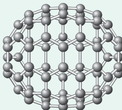
C_{70}
