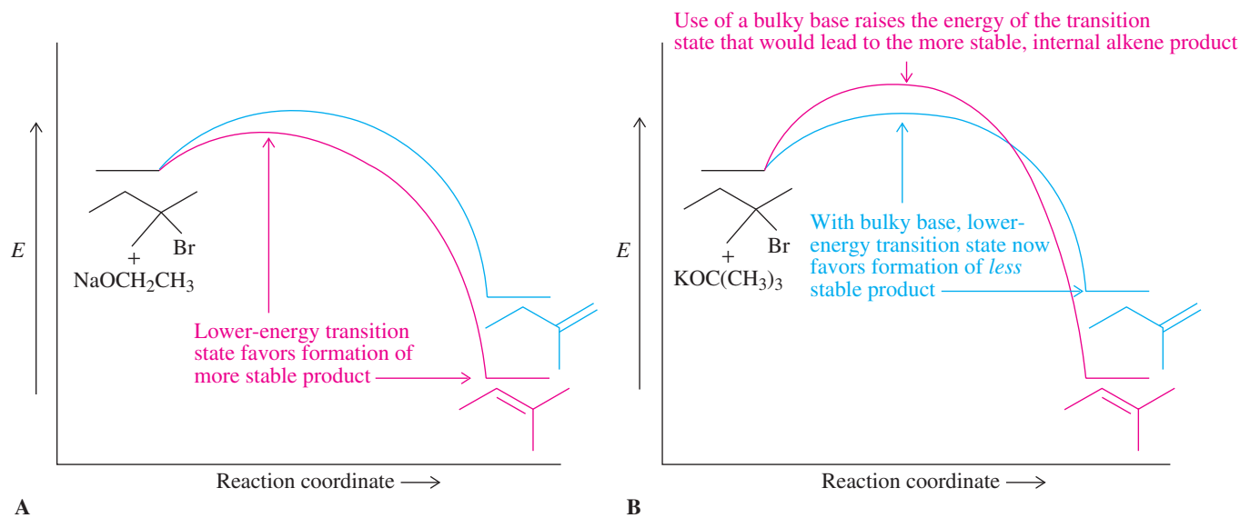
Figure 11-15 Potential energy diagrams for E2 reactions of 2-bromo-2-methylbutane with (A) sodium ethoxide (Saytzev rule) and (B) potassium tert -butoxide (Hofmann rule).
