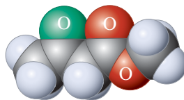
Methyl 3-oxobutanoate (Methyl acetoacetate) (A \beta -ketoester)
