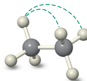
Staggered: More stable, because facing C–H bonds are at maximum distance (dashed lines)
