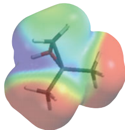
Protonated 2,2-dimethyloxacyclopropane
