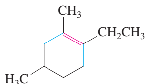
1-Ethyl-2,4-dimethylcyclohexene
