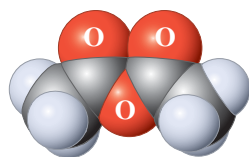
Acetic anhydride
