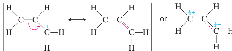
2-Propenyl (allyl) cation
