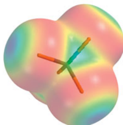
Tetrachloromethane
