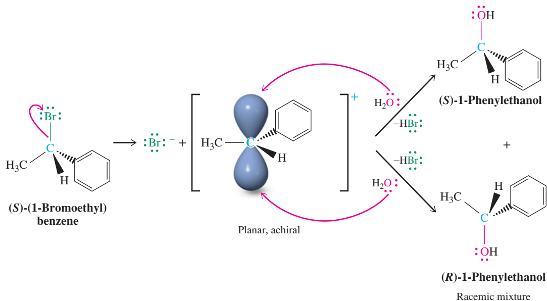
Figure 7-3 The mechanism of hydrolysis of ( S )-(1-bromoethyl)benzene explains the stereochemistry of the reaction. Initial ionization furnishes a planar, achiral carbocation. This ion, when trapped with water, yields racemic alcohol.
