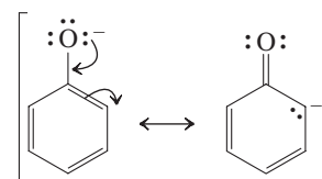
Phenoxide ion
