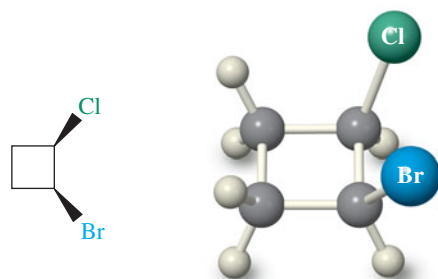
cis-1-Bromo-2-chlorocyclobutane
