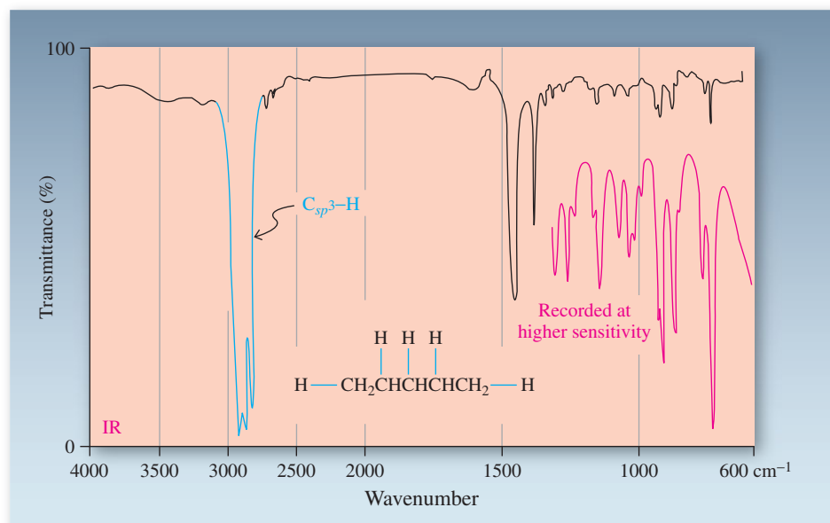
Figure 11-18 IR spectrum of pentane. Note the format: Wavenumber is plotted (decreasing from left to right) against percentage of transmittance. A 100% transmittance means no absorption; therefore “peaks” in an IR spectrum point downward . The spectrum shows absorbances at \bar{\nu}_{\text{C-H stretch}} = 2960, 2930, and 2870 \text{ cm}^{-1} ; \bar{\nu}_{\text{C-H bend}} = 1460, 1380, and 730 \text{ cm}^{-1} . The region between 600 and 1300 \text{ cm}^{-1} is also shown recorded at higher sensitivity (in red), revealing details of the pattern in the fingerprint region.
