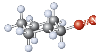
Cyclohexanecarbonitrile
