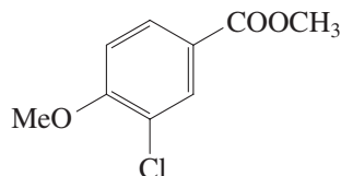
Compound 7
