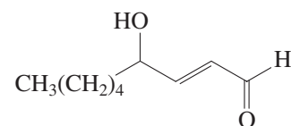
trans -4-Hydroxy-2-nonenal
