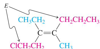
(E)-1-Chloro-3-ethyl-4-methyl-3-heptene
