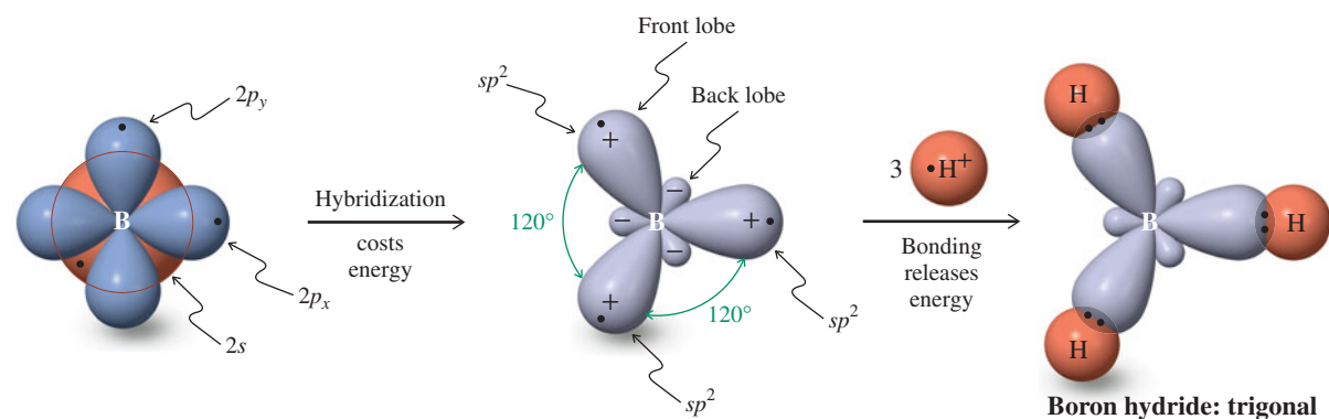
Figure 1-17 Hybridization in boron to create three sp^2 hybrids. The resulting bonding gives \text{BH}_3 a trigonal planar structure. There are three front lobes of one sign and three back lobes of opposite sign. The remaining p orbital ( p_z ) is perpendicular to the molecular plane (the plane of the page; one p_z lobe is above, the other below that plane) and has been omitted. In analogy to Figure 1-16B, the energy diagram for the hybridized boron features three singly occupied, equal-energy sp^2 levels and one remaining empty 2p level, in addition to the filled 1s orbital.
