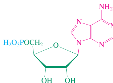
Adenylic acid
