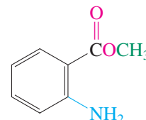
Methyl 2-aminobenzoate (Methyl anthranilate)
