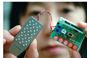
The world's smallest direct methanol fuel cell.
