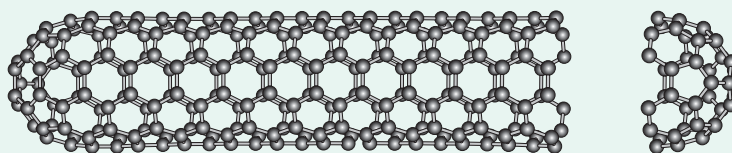
Carbon nanotube
