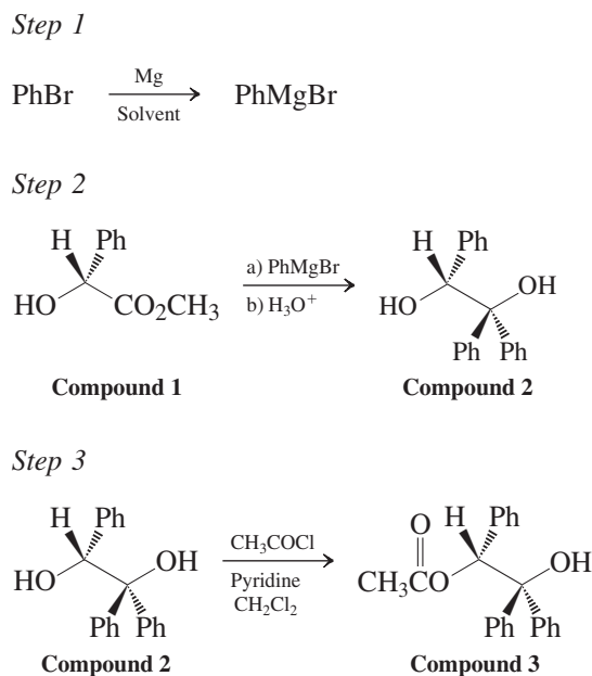
Figure 1 Synthesis of Compound 3 (Ph = phenyl, \text{C}_6\text{H}_5 –).
