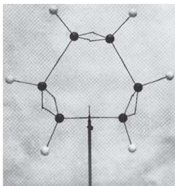
Kekulé's original model of benzene.
