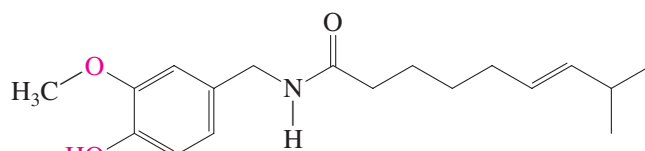
Capsaicin
