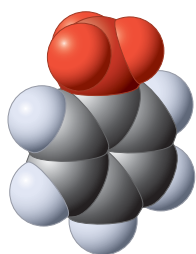
Methylbenzene (Toluene)
