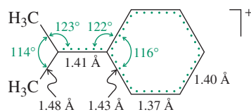
Figure 22-2 Structure of the 2-phenyl-2-propyl cation.
