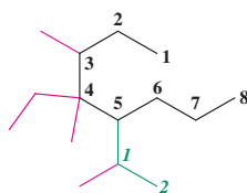
4-Ethyl-3,4-dimethyl-5-(1-methylethyl)octane
