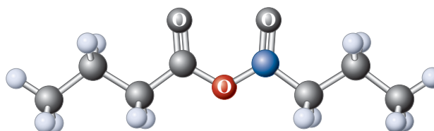
Butanoyl chloride
