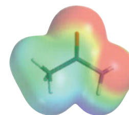
Acetamide
