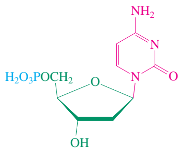
2'-Deoxycytidylic acid
