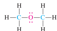
Methoxymethane (Dimethyl ether) (b.p. -23^\circ\text{C} )
