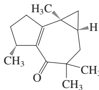
Africanone
