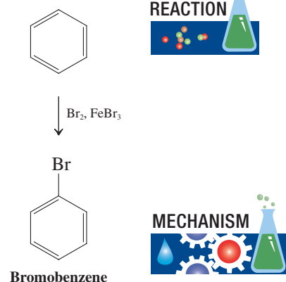
Bromobenzene
