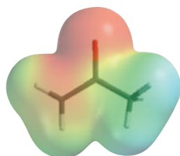
Acetone enolate
