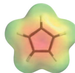
Cyclopentadienyl anion: aromatic
