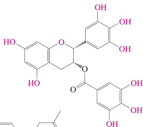
Epigallocatechin-3 gallate
