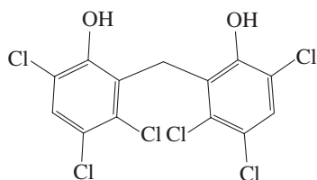
Hexachlorophene
