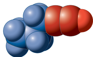
Propylacetylene
