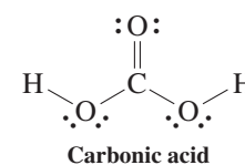
Carbonic acid
