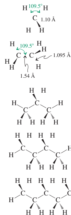
Figure 2-4 Hashed-wedged line structures of methane through pentane. Note the zigzag arrangement of the principal chain and two terminal hydrogens.
