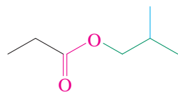
2-Methylpropyl propanoate (Isobutyl propionate)
