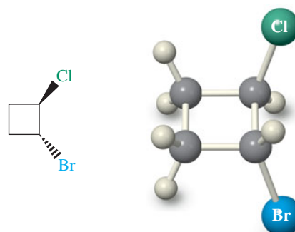
trans-1-Bromo-2-chlorocyclobutane
