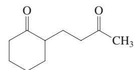
2-(3-Oxobutyl)cyclohexanone
