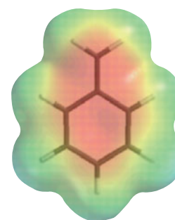
Phenylmethyl (benzyl) anion
