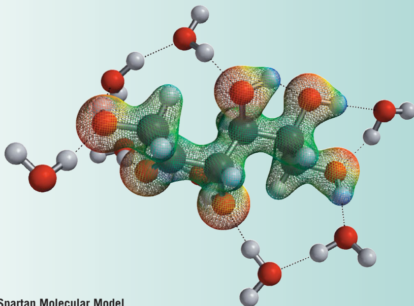
Spartan Molecular Model
