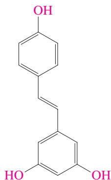
Resveratrol
