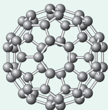
Buckminsterfullerene C_{60}
