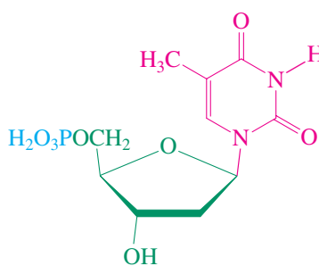
Thymidylic acid
