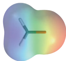
Formaldehyde
