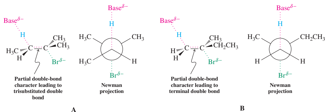
Figure 11-14 The two transition states leading to products in the dehydrobromination of 2-bromo-2-methylbutane. With unhindered base ( \text{CH}_3\text{CH}_2\text{O}^- \text{Na}^+ ), transition state A is preferred over transition state B because there are more substituents around the partial double bond (Saytzev rule). With hindered base [ (\text{CH}_3)_3\text{CO}^- \text{K}^+ ], transition state B is preferred over transition state A because there is less steric hindrance to abstraction of the primary hydrogens (Hofmann rule).
