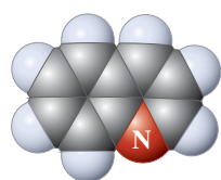
Quinoline
