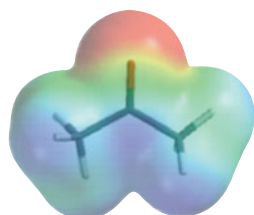
Acetone
