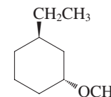
trans -1-Ethyl-3-methoxycyclohexane
