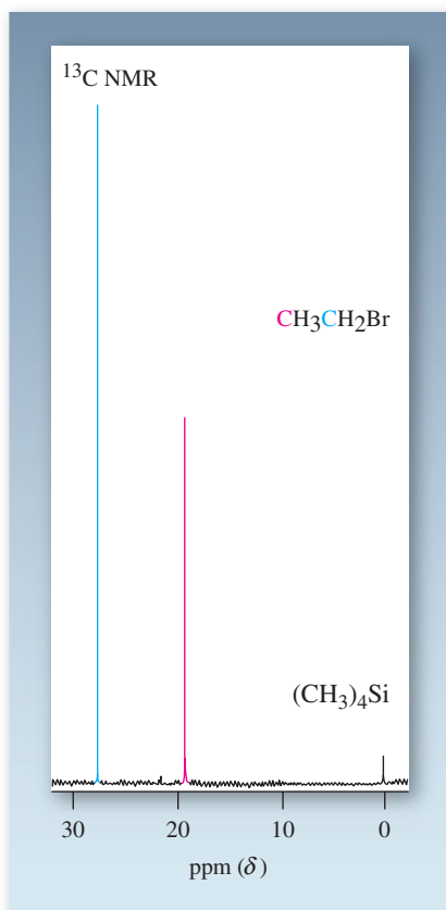
Figure 10-31 This 62.8-MHz ^{13}\text{C} NMR spectrum of bromoethane was recorded with broad-band decoupling at 250 MHz. All lines simplify to singlets, including the absorption for (\text{CH}_3)_4\text{Si} .
