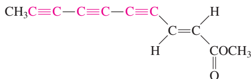
Dehydromatricaria ester
