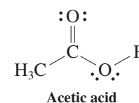
Acetic acid
