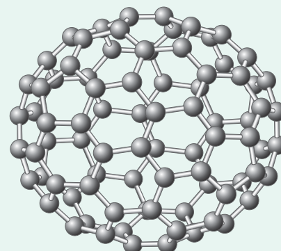
Chiral C_{84}
