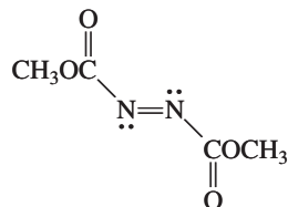
Dimethyl azodicarboxylate
