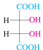
meso-Tartaric acid (Not optically active)
