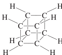
Cubane
