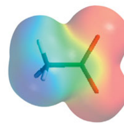
Acetate ion
