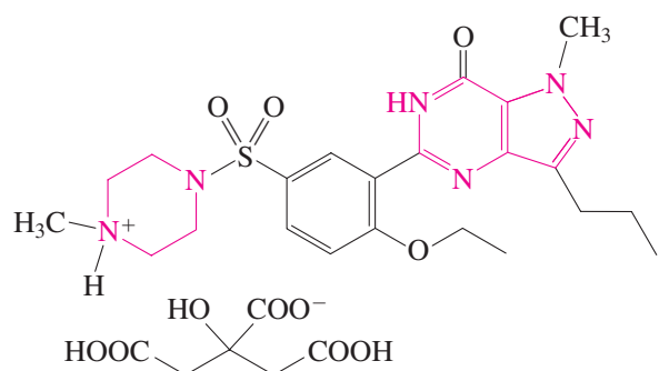
Viagra (Sildenafil citrate)
