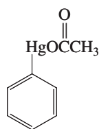
Phenylmercury acetate
