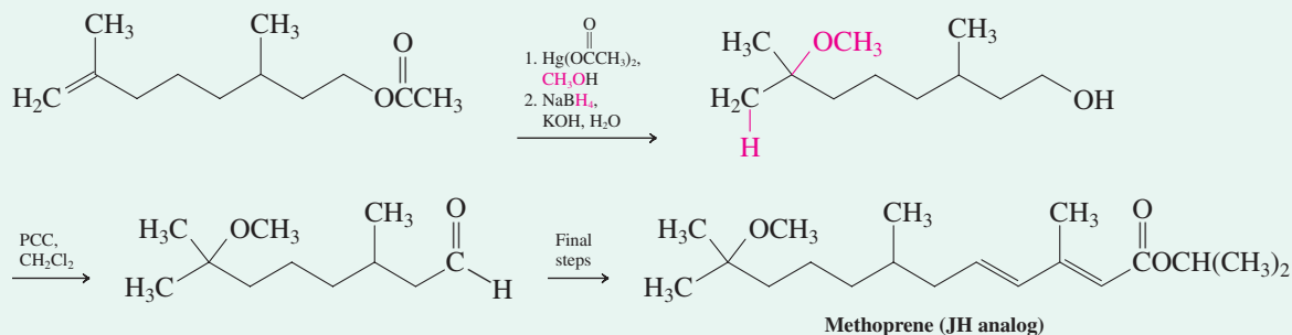
Juvenile hormone
