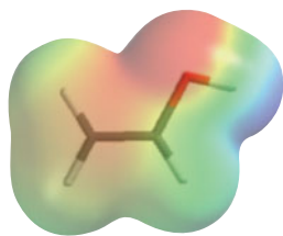
Ethenol
