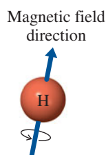
Spinning proton
