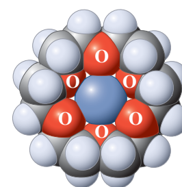
Space-filling model of the cation [\text{K}^+ \text{18-crown-6}] .
