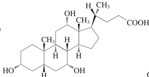
Cholic acid
