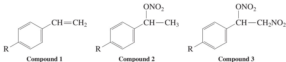
Figure 1 Reactants and products.
