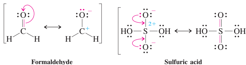
Formaldehyde
