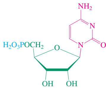
Cytidylic acid
