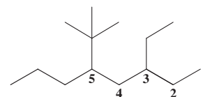
5-(1,1-Dimethylethyl)-3-ethyloctane
