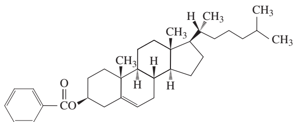
Cholesteryl benzoate
