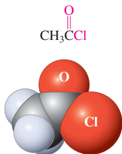
Acetyl chloride
