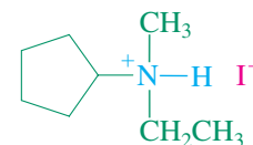
Cyclopentylethylmethylammonium iodide
