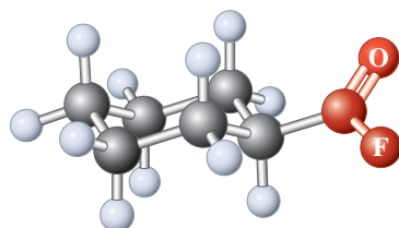
Cyclohexanecarbonyl fluoride
