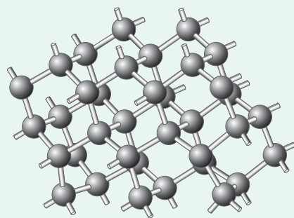
Diamond
