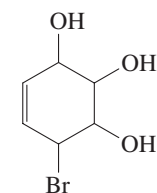
Bromoconduritol
