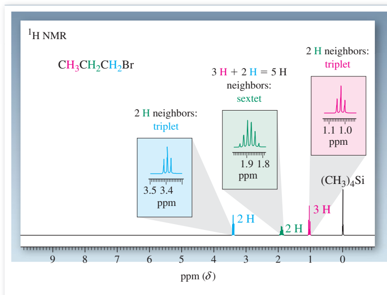
Figure 10-27 300-MHz ^1\text{H} NMR spectrum of 1-bromopropane.
