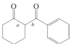
2-Benzoylcyclohexanone
