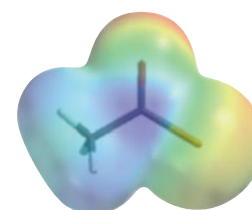
Acetyl chloride
