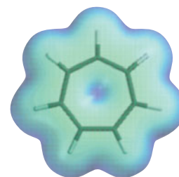
Cycloheptatrienyl cation: aromatic
