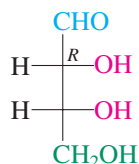
Structure 1 (D-Erythrose)
