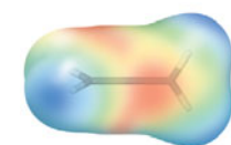
1,2-Propadiene (Allene, nonconjugated)
