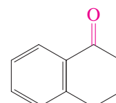
1-Oxo-1,2,3,4-tetrahydronaphthalene (1-Tetralone)
