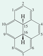
trans -15,16-Dihydropyrene
