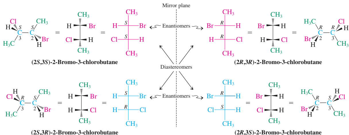
Figure 5-7 The four stereoisomers of 2-bromo-3-chlorobutane. Each molecule is the enantiomer of one of the other three (its mirror image) and is at the same time a diastereomer of each of the remaining two. For example, the 2R,3R isomer is the enantiomer of the 2S,3S compound and is a diastereomer of both the 2S,3R and the 2R,3S structures. Notice that two structures are enantiomers only when they possess the opposite configuration at every stereocenter.
