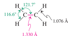
Figure 11-1 Molecular structure of ethene.
