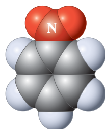
Benzenamine (Aniline) (A primary amine)
