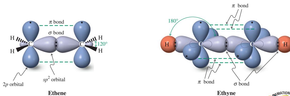
Figure 1-21 The double bond in ethene (ethylene) and the triple bond in ethyne (acetylene).
