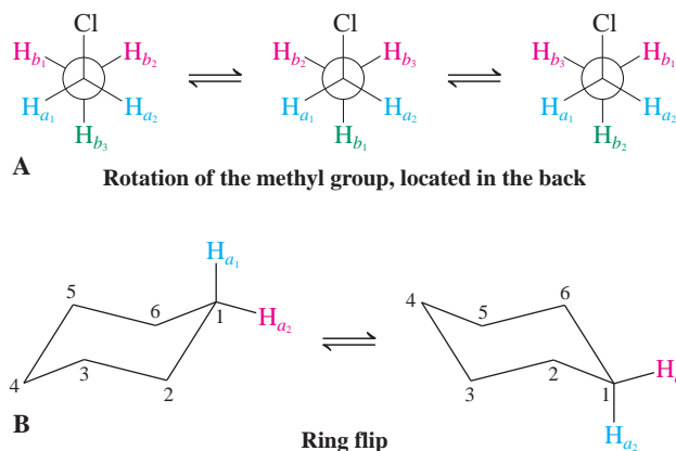
Figure 10-14 (A) Newman projections of chloroethane. In the initial conformation, H_{b_1} and H_{b_2} are located gauche and H_{b_3} anti to the chlorine, and therefore are not in the same environments. However, fast rotation moves each type of H through all positions, thus averaging all the methyl hydrogens on the NMR time scale. (B) In any given conformation of cyclohexane, the axial hydrogens are different from the equatorial ones. However, conformational flip is rapid on the NMR time scale, equilibrating axial and equatorial hydrogens, so only one average signal is observed. Colors are used here to distinguish among environments and thus to indicate distinct chemical shifts.
