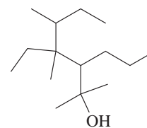
Alcohol 2
