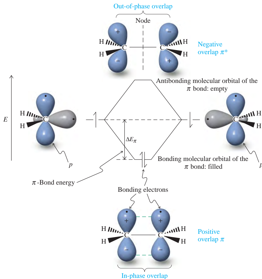
Figure 11-4 Compare this picture of the formation of the \pi bond in ethene with Figure 11-3. In-phase interaction between two parallel p orbitals (containing one electron each; shown in blue) results in positive overlap and a filled bonding \pi orbital. The representation of this orbital indicates the probability of finding the electrons between the carbons above and below the molecular plane. Because \pi overlap is less effective than \sigma , the stabilization energy, \Delta E_\pi , is smaller than \Delta E_\sigma . The \pi bond is therefore weaker than the \sigma bond. The out-of-phase interaction results in the antibonding molecular orbital \pi^* .
