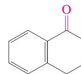
1-Oxo-1,2,3,4-tetrahydronaphthalene (1-Tetralone)
