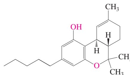
Tetrahydrocannabinol
