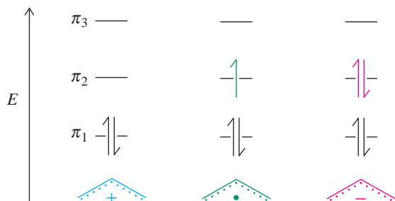
Figure 14-3 The Aufbau principle is used to fill up the \pi molecular orbitals of 2-propenyl (allyl) cation, radical, and anion. In each case, the total energy of the \pi electrons is lower than that of three noninteracting p orbitals. Partial cation, radical, or anion character is present at the end carbons in these systems, a result of the location of the lobes in the \pi_2 molecular orbital.
