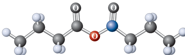
Butanoyl chloride
