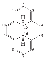
trans -15,16-Dihydropyrene
