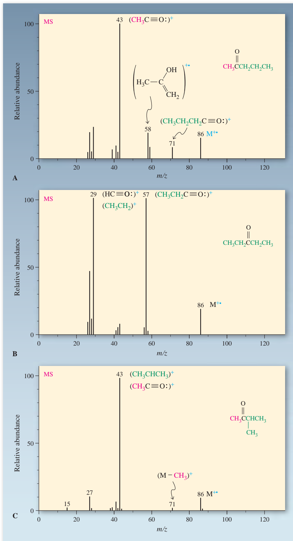
Figure 17-7 Mass spectra of (A) 2-pentanone, showing two peaks for \alpha cleavage and one for McLafferty rearrangement; (B) 3-pentanone, showing only a single \alpha cleavage peak because of symmetry; and (C) 3-methyl-2-butanone, showing two \alpha cleavages.
