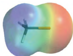
Chloromethane
