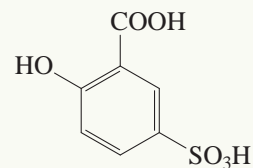
Sulfosalicylic acid
