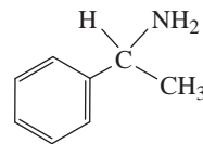
1-Phenylethanamine
