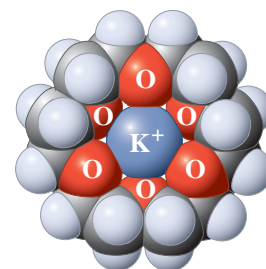
Space-filling model of the cation [\text{K}^+ \text{18-crown-6}] .
