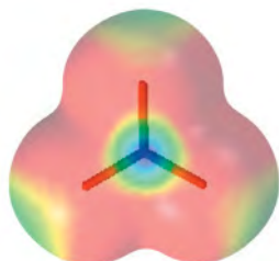
Carbonate ion
