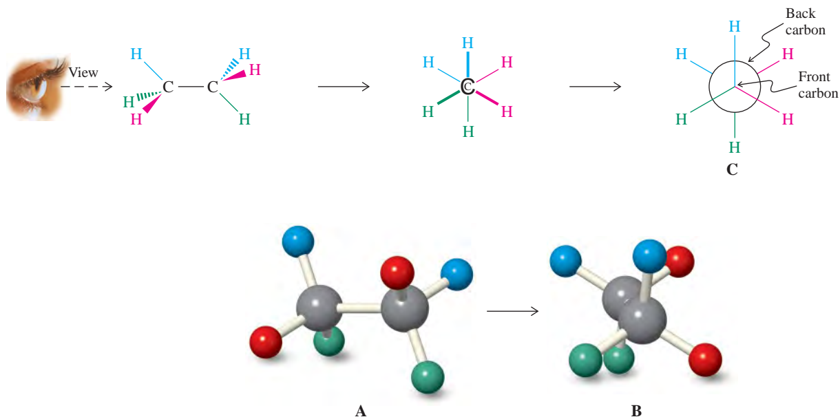
Figure 2-8 Representations of ethane. (A) Side-on views of the molecule. (B) End-on views of ethane, showing the carbon atoms directly in front of each other and the staggered positions of the hydrogens. (C) Newman projection of ethane derived from the view shown in (B). The “front” carbon is represented by the intersection of the bonds to its three attached hydrogens. The bonds from the remaining three hydrogens connect to the large circle, which represents the “back” carbon.
