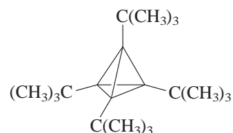
Tetrakis(1,1-dimethylethyl)-tetrahedrane
