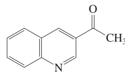
3-Acetylquinoline
