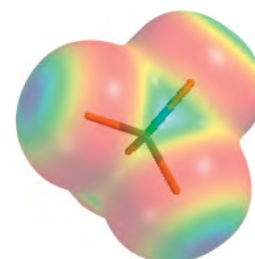
Tetrachloromethane
