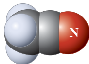
Ethanenitrile (Acetonitrile)
