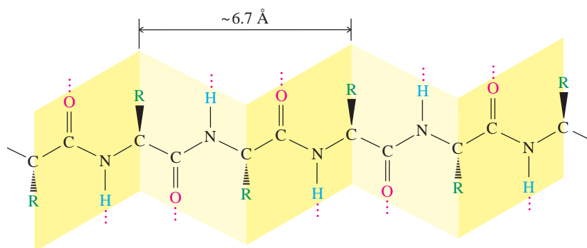
Figure 26-3 (A) The pleated sheet, or \beta configuration, which is held in place by hydrogen bonds (dotted lines) between two polypeptide strands. (After “Proteins,” by Paul Doty, Scientific American , September 1957. Copyright © 1957, Scientific American, Inc.) (B) The peptide bonds define the individual pleats (shaded in yellow); the positions of the side chains, R, are alternately above and below the planes of the sheets. The dotted lines indicate hydrogen bonds to a neighboring chain or to water.
