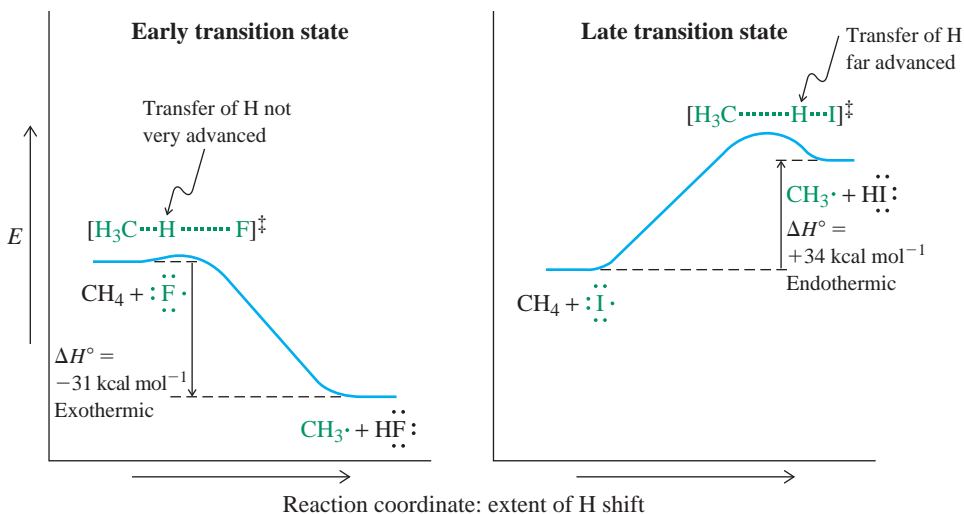
Figure 3-8 Potential-energy diagrams: (left) the reaction of a fluorine atom with CH 4 , an exothermic process with an early transition state; and (right) the reaction of an iodine atom with CH 4 , an endothermic transformation with a late transition state. Both are thus in accord with the Hammond postulate.
