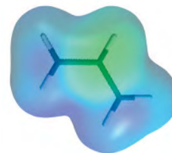
2-Propenyl cation
