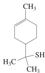
( R,S )-2-(4-Methyl-3-cyclohexenyl)-2-propanethiol
