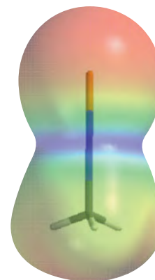
Methylmagnesium chloride
