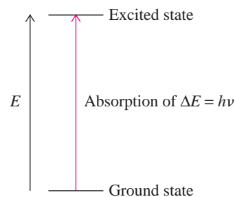
Figure 10-1 Absorption of energy occurs when incident radiation has exactly the right frequency \nu so that its energy h\nu equals the energy difference \Delta E between the ground state and the excited state of a molecule [ \nu , frequency of absorbed radiation; h (Planck’s constant) = 6.626 \times 10^{-34} J s].
