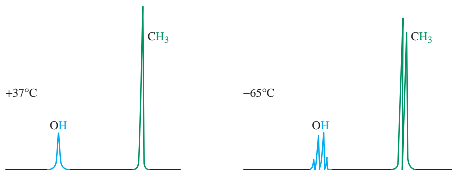
Figure 10-29 Temperature dependence of spin-spin splitting in methanol. The singlets at 37^\circ\text{C} illustrate the effect of fast proton exchange in alcohols. (After H. Günther, NMR-Spektroskopie , Georg Thieme Verlag, Stuttgart, 1973.)
