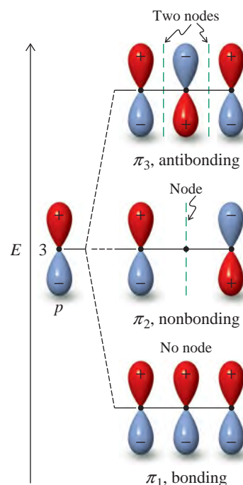
Figure 14-2 The three \pi molecular orbitals of 2-propenyl (allyl), obtained by combining three adjacent atomic p orbitals. Note the drop in energy of the bonding molecular orbital \pi_1 , reflecting the increased stability of the system. Molecular orbital \pi_2 remains at the same level as the starting p orbitals and is therefore called a nonbonding molecular orbital.
