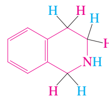
1,2,3,4-Tetrahydroisoquinoline
