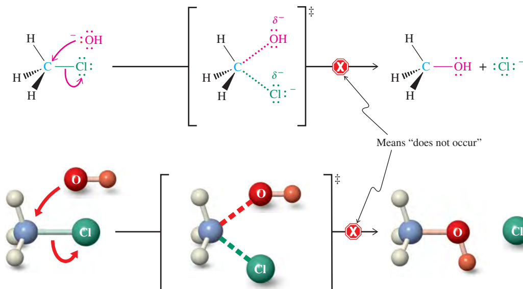
Figure 6-2 Hypothetical frontside nucleophilic substitution (does not occur). The (hypothetical) transition state is enclosed in brackets and labeled with the ‡ symbol.
