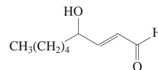
trans -4-Hydroxy-2-nonenal
