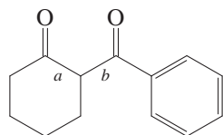
2-Benzoylcyclohexanone
