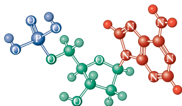
2'-Deoxyadenylic acid
