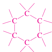
A carbocycle
