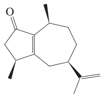
Rotundone
