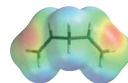
1,4-Pentadiene (Nonconjugated)
