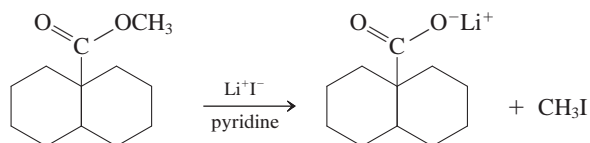
Pyridine
