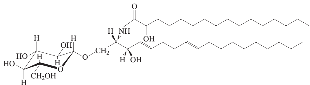
Glucosyl cerebroside
