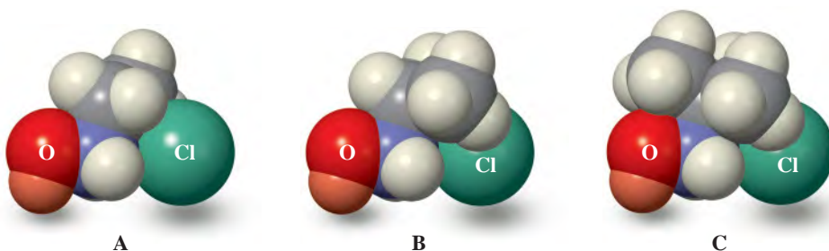
Figure 6-10 Hashed-wedged line and space-filling renditions of the transition states for S N 2 reactions of hydroxide ion with (A) 1-chloropropane, (B) 1-chloro-2-methylpropane, and (C) 1-chloro-2,2-dimethylpropane. Increasing steric hindrance from a second gauche interaction reduces the rate of reaction in (B). S N 2 reactivity in (C) is eliminated almost entirely because a methyl group prevents backside attack by the nucleophile in all accessible conformations of the substrate. (See also Figures 6-8 and 6-9.)
