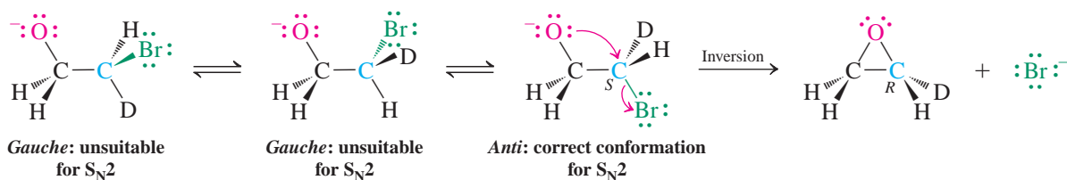
Figure 9-6 Only the anti conformation of a 2-bromoalkoxide allows for oxacyclopropane formation. The two gauche conformers cannot undergo intramolecular backside attack at the bromine-bearing carbon.
