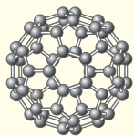
Buckminsterfullerene C_{60}
