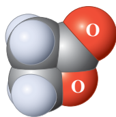
\beta -Propiolactone
