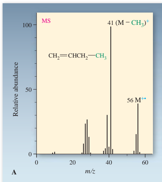
Figure 11-29 Mass spectra of (A) 1-butene, showing a peak at m/z = 41 from cleavage to give the resonance-stabilized 2-propenyl (allyl) cation; (B) 2-hexene, showing similar cleavage between C4 and C5 to give the 2-butenyl cation, with m/z = 55 .
