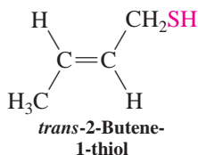
trans -2-Butene-1-thiol
