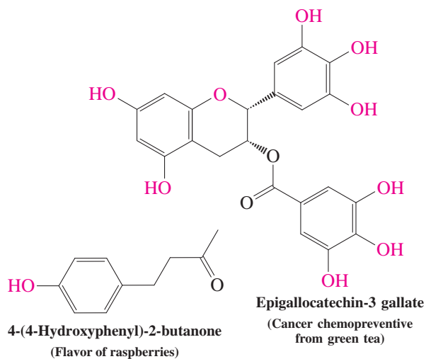
Green tea.
