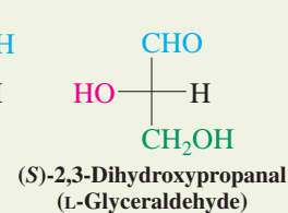
Fischer projections
