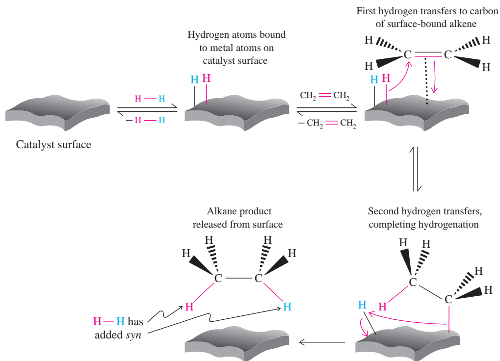
Figure 12-1 Mechanism of catalytic hydrogenation of ethene to produce ethane. The hydrogens bind to the catalyst surface and are delivered to the carbons of the surface-adsorbed alkene.
