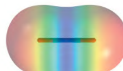
Carbon dioxide
