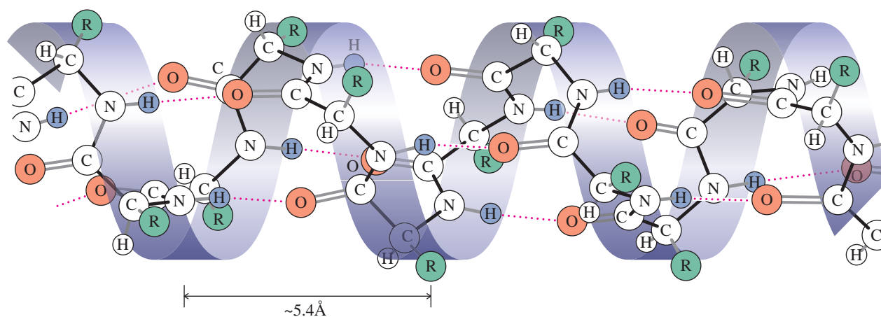
Figure 26-4 The \alpha helix, in which the polymer chain is arranged as a right-handed spiral held rigidly in shape by intramolecular hydrogen bonds (red dotted lines). (After “Proteins,” by Paul Doty, Scientific American , September 1957. Copyright © 1957, Scientific American, Inc.)
