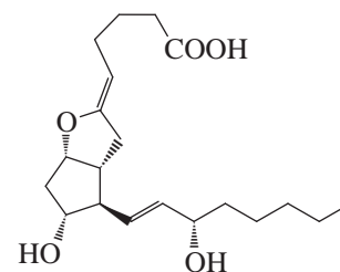
Prostacyclin I_2
