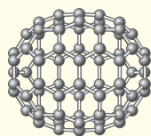
C_{70}
