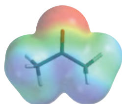
Acetone
