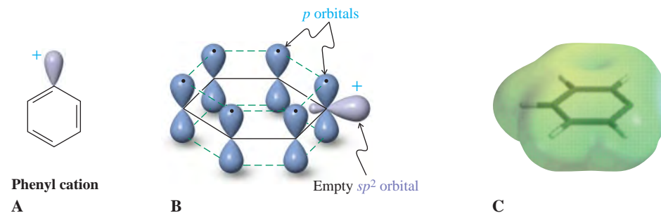
Figure 22-5 (A) Line structure of the phenyl cation. (B) Orbital picture of the phenyl cation. The alignment of its empty sp^2 orbital is perpendicular to the six- \pi -electron framework of the aromatic ring. As a result, the positive charge is not stabilized by resonance. (C) The electrostatic potential map of the phenyl cation, shown at an attenuated scale for better contrast, pinpoints much of the positive charge (blue edge on the right) as located in the plane of the six-membered ring.
