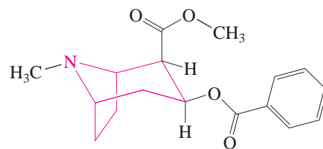
Cocaine
