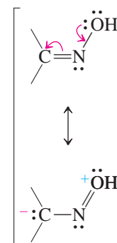
Resonance stabilization in oximes
