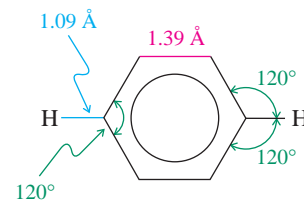
Figure 15-1 The molecular structure of benzene. All six C–C bonds are equal; all bond angles are 120^\circ .
