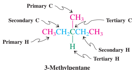
3-Methylpentane
