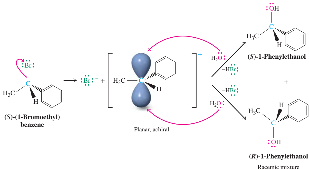
Figure 7-3 The mechanism of hydrolysis of (S)-(1-bromoethyl)benzene explains the stereochemistry of the reaction. Initial ionization furnishes a planar, achiral carbocation. This ion, when trapped with water, yields racemic alcohol.
