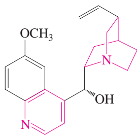
Quinine
