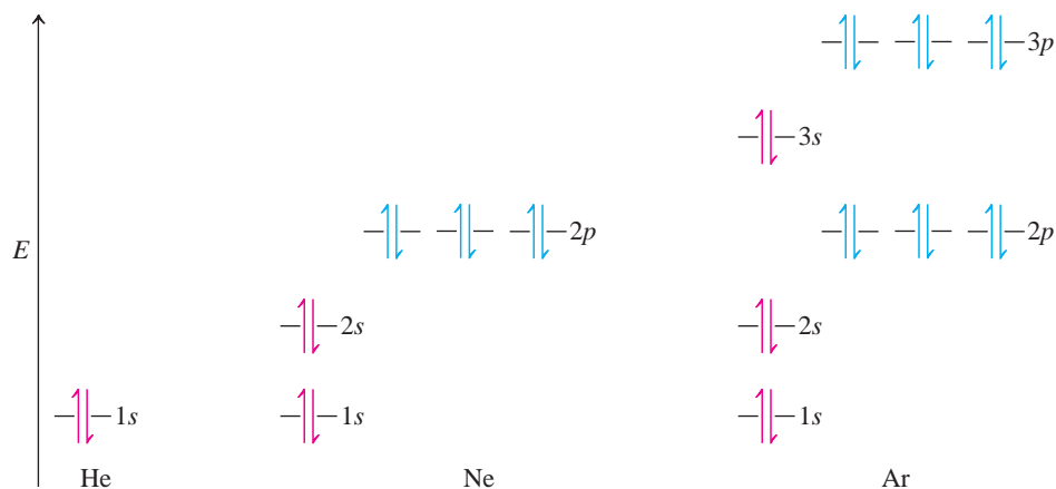
Figure 1-10 Closed-shell configurations of the noble gases helium, neon, and argon.
