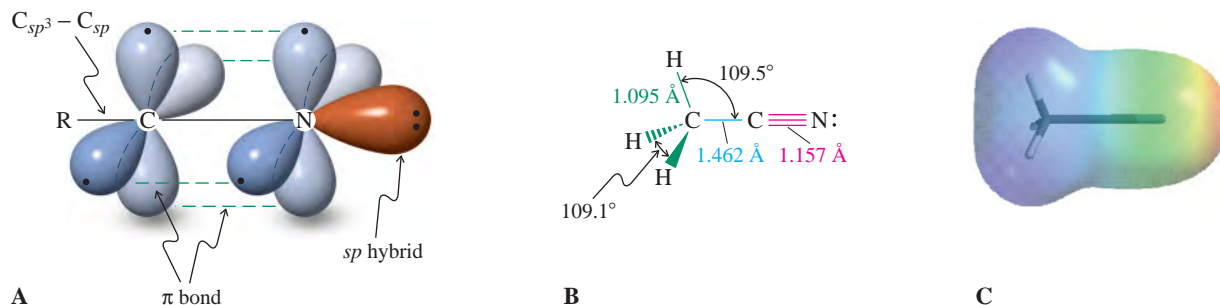
Figure 20-3 (A) Orbital picture of the nitrile group, showing the sp hybridization of both atoms in the \text{C}\equiv\text{N} function. (B) Molecular structure of ethanenitrile (acetoneitrile), which is similar to that of the corresponding alkyne. (C) Electrostatic potential map of ethanenitrile, depicting the positively polarized cyano carbon (blue) and the relatively negatively polarized nitrogen (green) with its lone electron pair (red).
