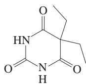
Veronal
