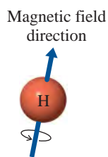
Spinning proton
