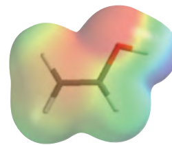
Ethenol
