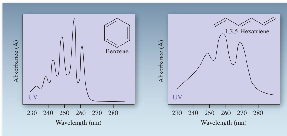
Figure 15-6 The distinctive ultraviolet spectra of benzene: \lambda_{\max}(\epsilon) = 234(30) , 238(50) , 243(100) , 249(190) , 255(220) , 261(150) nm; and 1,3,5-hexatriene: \lambda_{\max}(\epsilon) = 247(33,900) , 258(43,700) , 268(36,300) nm. The extinction coefficients \epsilon of the absorptions of 1,3,5-hexatriene are very much larger than those of benzene; therefore the spectrum at the right was taken at lower concentration.
