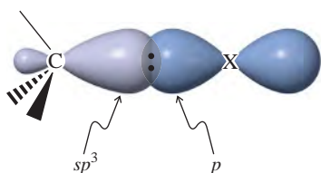
Figure 6-1 Bond between an alkyl carbon and a halogen. The size of the p orbital is substantially larger than that shown for X = \text{Cl, Br, or I} .
