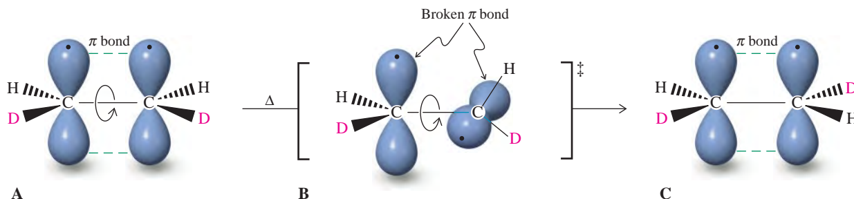
Figure 11-6 Thermal isomerization of cis -dideuterioethene to the trans isomer requires breaking the \pi bond. The reaction proceeds from starting material (A) through rotation around the C–C bond until it reaches the point of highest energy, the transition state (B). At this stage, the two p orbitals used to construct the \pi bond are perpendicular to each other. Further rotation in the same direction results in a product in which the two deuterium atoms are trans (C).
