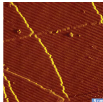
Scanning tunneling microscope (STM) image of a catalytic Pt surface. STM provides pictures at atomic resolution (the bar at the bottom right indicates 5 \text{ nm} = 50 \text{ \AA} ). You can see the highly ordered patterns of parallel arrays of Pt atoms in brown. The yellow "crosslines" indicate steps on the surface, on which much of the catalytic activity takes place. (Courtesy Professor Gabor A. Somorjai and Dr. Feng Tao, University of California at Berkeley.)
