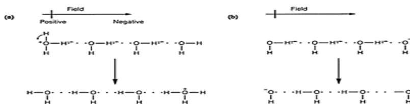
Fig. 1. The Grotthus mechanism for (a) \text{H}^+ ; (b) \text{OH}^- ion motion in water. The arrows indicate the concerted proton movement when the field is applied.
