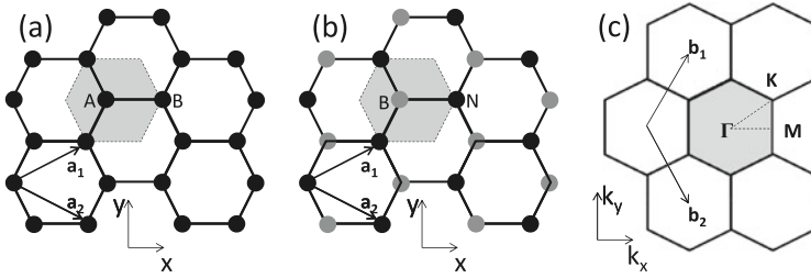
Fig. 1.6 Real space lattice for a hexagonal monolayer of a graphene and b boron nitride. c The reciprocal space lattice for a 2D hexagonal lattices generally. The shaded hexagon in a is the Wigner–Seitz unit cell in real space and in c is the corresponding Brillouin zone in reciprocal space
