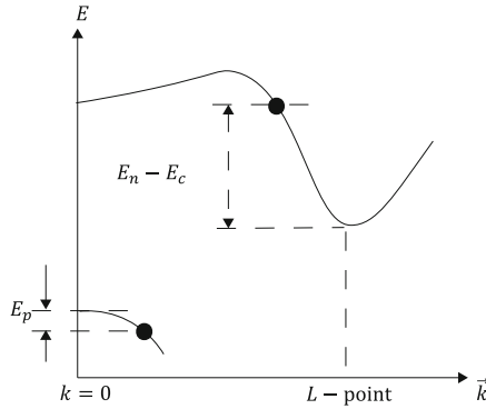
Fig. 18.10 Schematic diagram of an indirect transition showing the notation used in the text. E_c is the energy of the L -point conduction band at wave vector k_c , while E_g is the thermal gap energy. The valence band maximum E_v is taken as the zero of energy. E_n and (\mathbf{k}_n - \mathbf{k}_c) , respectively, denote the energy and momentum of an excited electron, while E_p and \mathbf{k}_p , respectively, denote the corresponding parameters for the holes near \mathbf{k} = 0 . It is customary to place the zero of energy at the valence band maximum
