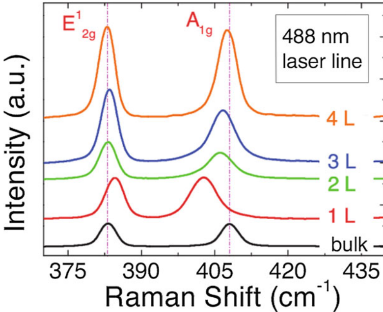
Fig. 22.15 Raman spectra of MoS 2 of various thicknesses. The left and right dashed lines indicate the positions of the E' 2g and A 1g peaks in bulk MoS 2 , respectively (Taken from Li et al. (2012))
