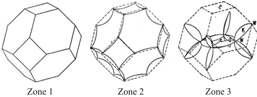
Fig. 4.8 The three valence electrons for aluminum occupy three Brillouin zones. Zone 1 is completely occupied. Zone 2 is nearly filled with electrons and is best described as a hole surface, where the holes occupy the interior portion of the second zone, shown in the figure. Zone 3 is a complex electron structure with occupied electron states near the Brillouin zone boundaries, and the occupied states are shown only in part for clarity. Reprinted with permission from Physical Review, vol. 118 p. 1190 Copyright (1960) American Physical Society
