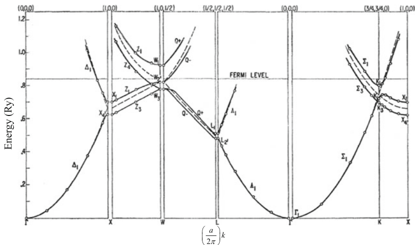
Fig. 4.7 Electronic energy band diagram for aluminum which is metallic and crystallizes in a FCC structure. The dashed lines correspond to the free electron model and the solid curves include the effect of the periodic potential V(\mathbf{r}) . Reprinted with permission from Physical Review, vol. 125 p. 109 Copyright (1962) American Physical Society
