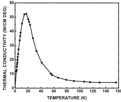
Fig. 8.1 The temperature dependence of the thermal conductivity of copper. Note that both \kappa and T are plotted on linear scales. At low temperatures where the phonon density is low, the thermal transport is by electrons predominantly, while at high temperatures, thermal transport by phonons becomes more important.
