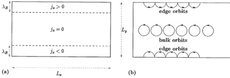
Fig. 14.7 Edge states and the orbits of carriers. a The edge regions shown here are defined by the characteristic length \lambda_B = (\hbar/eB)^{1/2} . Along each edge, b shows that all complete orbits give rise to a current j_x in the same direction, but the current direction is opposite for the two edges in (b) . The bulk orbits, however, do not give rise to a current j_x
