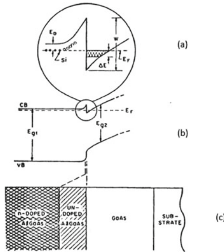
Fig. 14.9 a Schematic diagram of a modulation-doped n -type semiconductor GaAs/ \text{Al}_x\text{Ga}_{1-x}\text{As} heterostructure and of its energy band structure. b CB and VB here refer to the conduction band (CB) and valence band (VB) edges; E_{g1} and E_{g2} are, respectively, the energy gaps of the \text{Al}_x\text{Ga}_{1-x}\text{As} and GaAs regions, while \Delta E in (a) is the energy corresponding to the zero-magnetic-field filling of the lowest quantum subband of the two-dimensional electron gas, and E_F is the Fermi energy. W is the step height (band offset energy) between the GaAs conduction band and the \text{Al}_x\text{Ga}_{1-x}\text{As} conduction band at the interface. The two-dimensional electron gas in (a) lies in the GaAs region close to the undoped \text{Al}_x\text{Ga}_{1-x}\text{As} (see c showing the lowest diagram). The dopants used to introduce the n -type carriers are located in the region labelled n -doped AlGaAs
