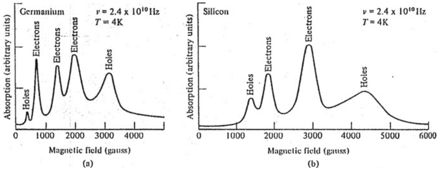
Fig. 13.2 Historic cyclotron resonance signals in the semiconductors a germanium and b silicon. The magnetic field lies in a (110) plane and makes an angle with the [001] axis of 60^\circ for the spectrum shown for Ge, and 30^\circ for the spectrum shown for Si. (From G. Dresselhaus, et al., Phys. Rev. 98 , 368 (1955).)
